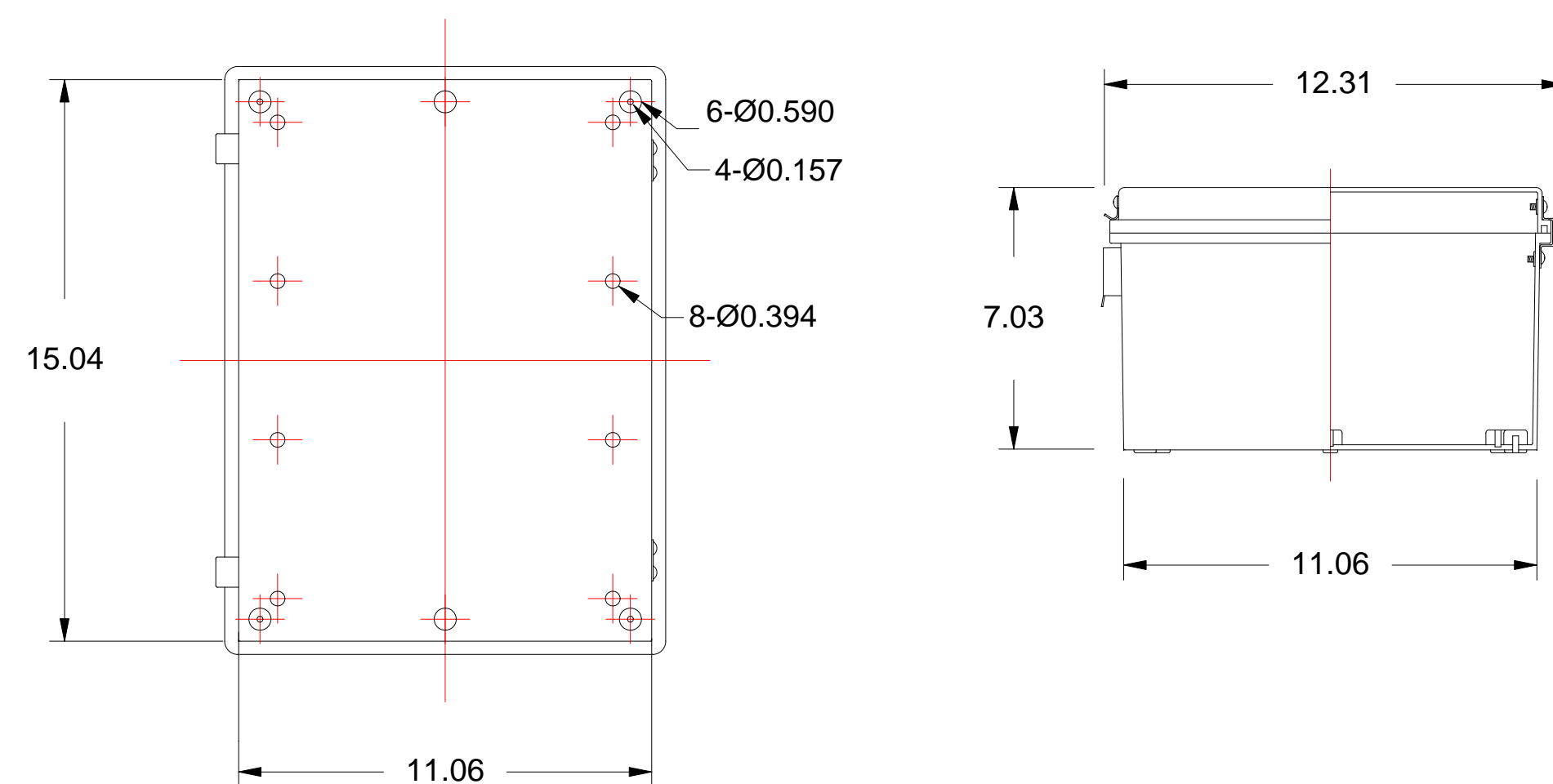
BOTTOM VIEW
