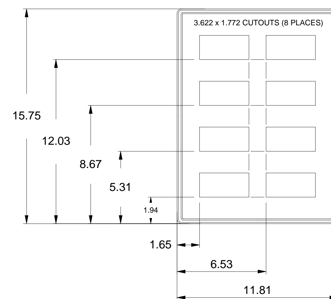
CUTOUT VIEW
