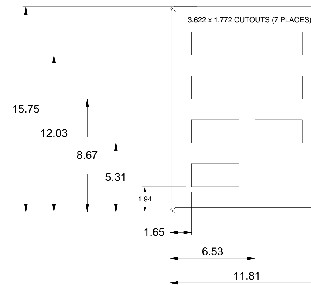
CUTOUT VIEW
