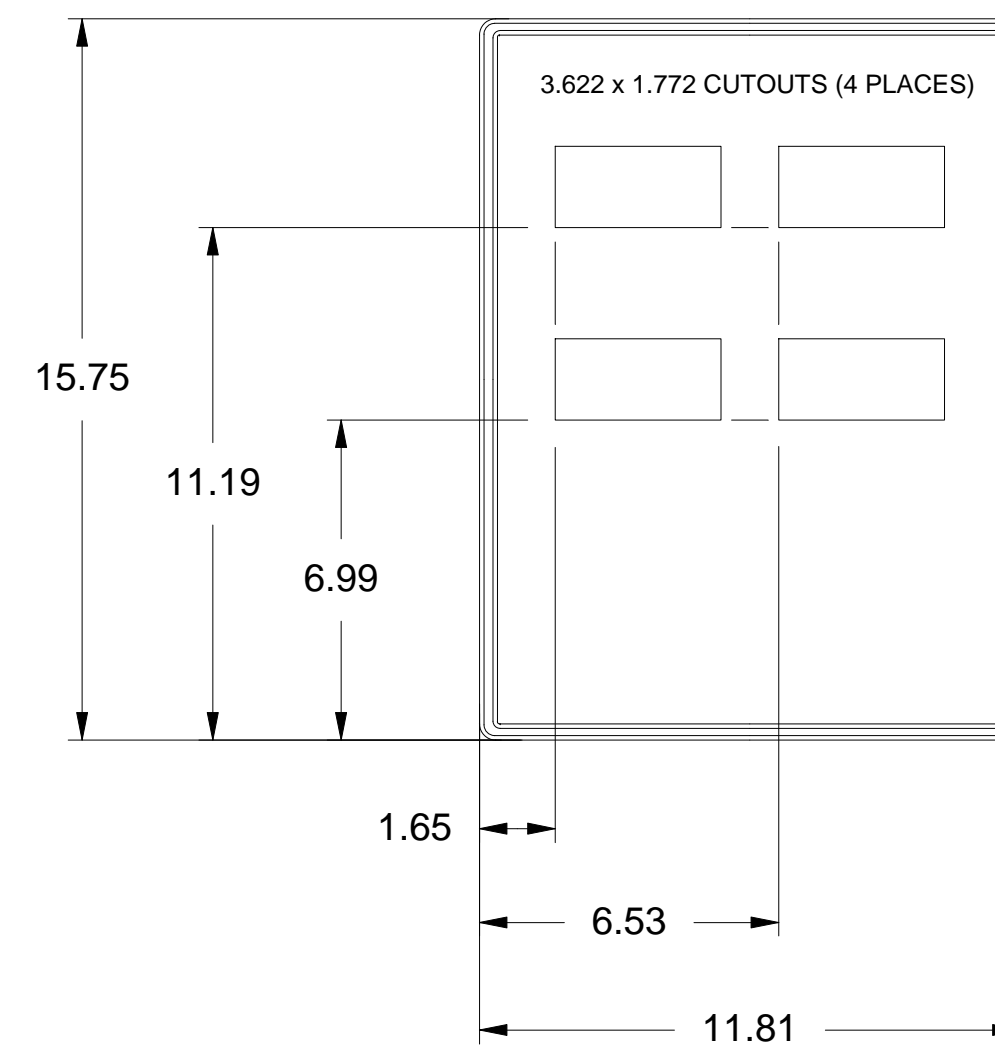
CUTOUT VIEW
