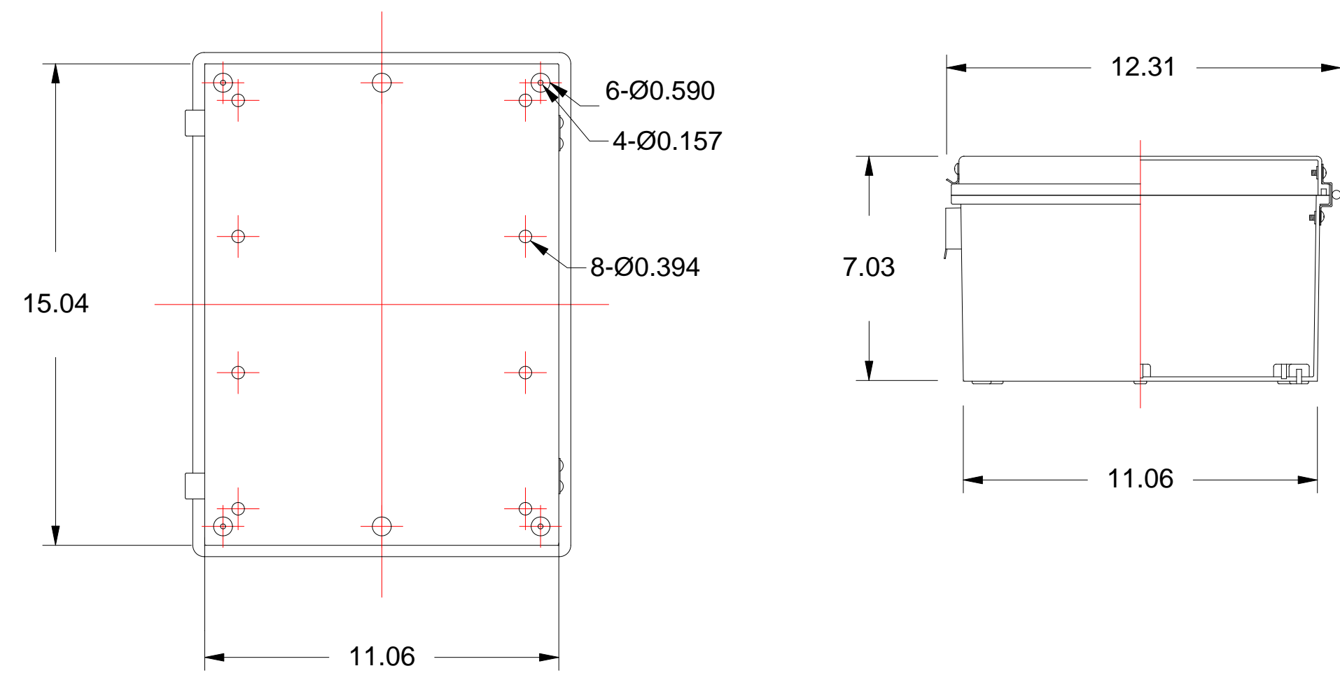
BOTTOM VIEW
