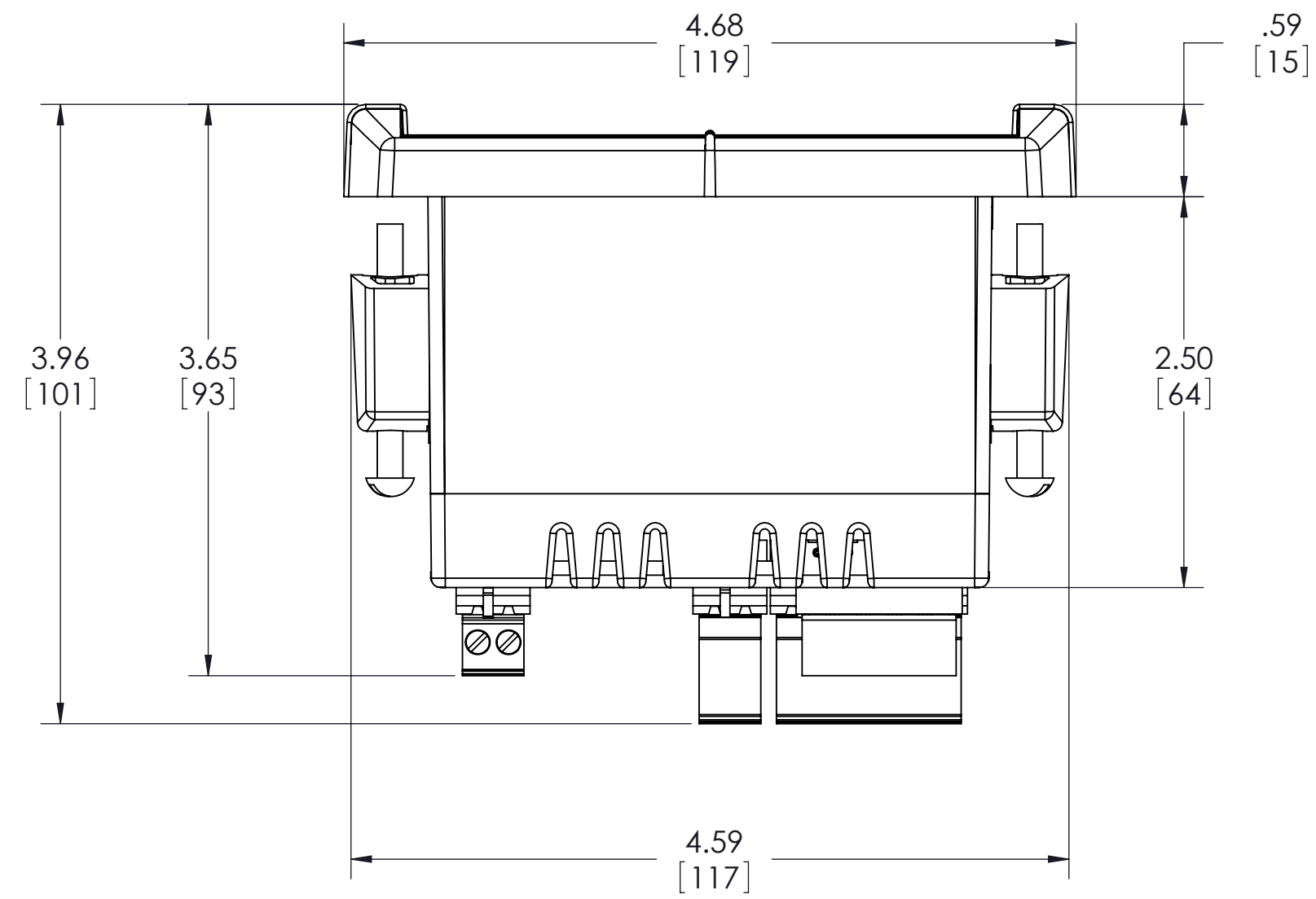
BOTTOM VIEW
