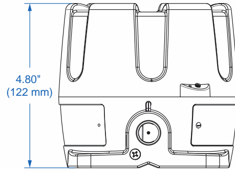
Figure 3. Enclosure Dimensions – Bottom View
