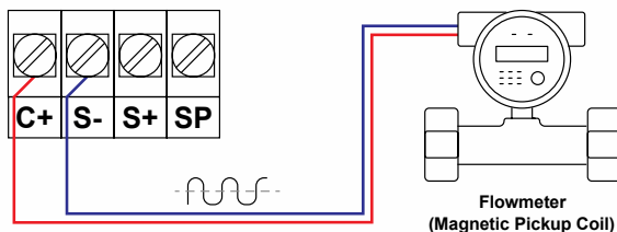
Figure 18. Self-Powered Magnetic Pickup Flowmeter (Coil)
