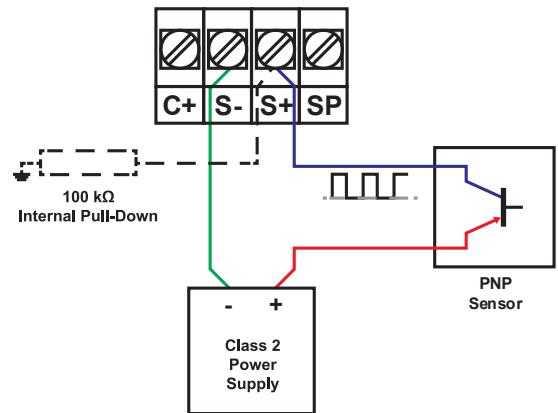
Figure 21. PNP Sensor with External Power
