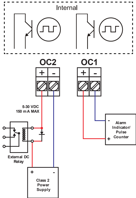
Figure 29. Open Collector Output Connections
