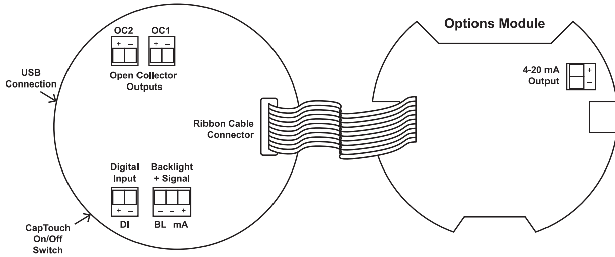
Figure 6. Connector Labeling for PD6928-GP-PL-L3N
