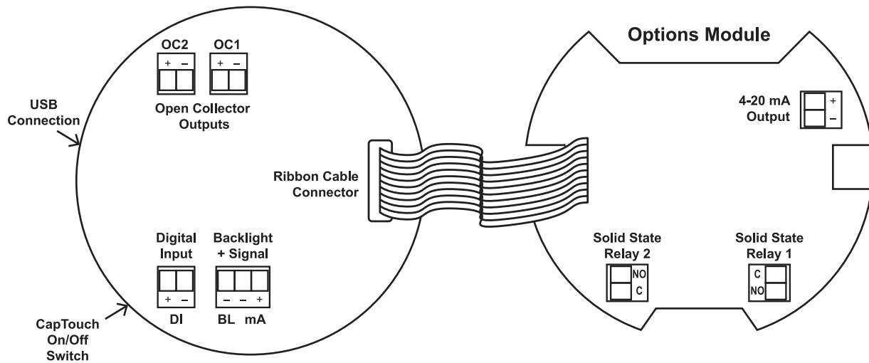
Figure 7. Connector Labeling for PD6928-GP-PL-L5N
