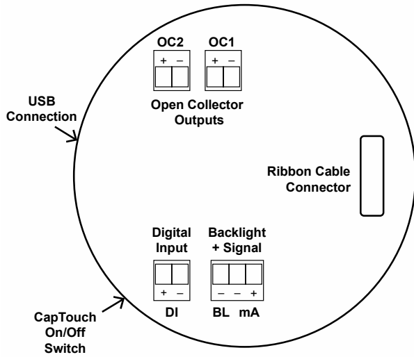
Figure 4. Connector Labeling for PD6928-GP-PL-LNN
