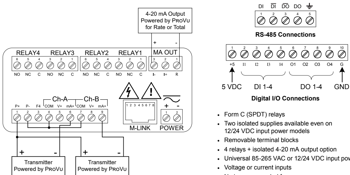
Connections for PD8-6262-6H7 & PD8-6262-7H7
